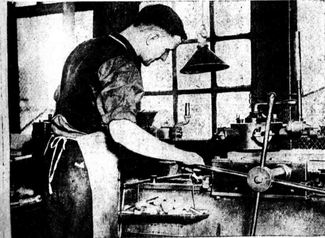
THREADING and putting seat on swan-neck faucets with a turret lathe at Thomas Savill's Sons, Thirteenth and Wallace streets. The operator, William Zerweck, of 2244 North Carlisle street, threads about 350 faucets a day.
