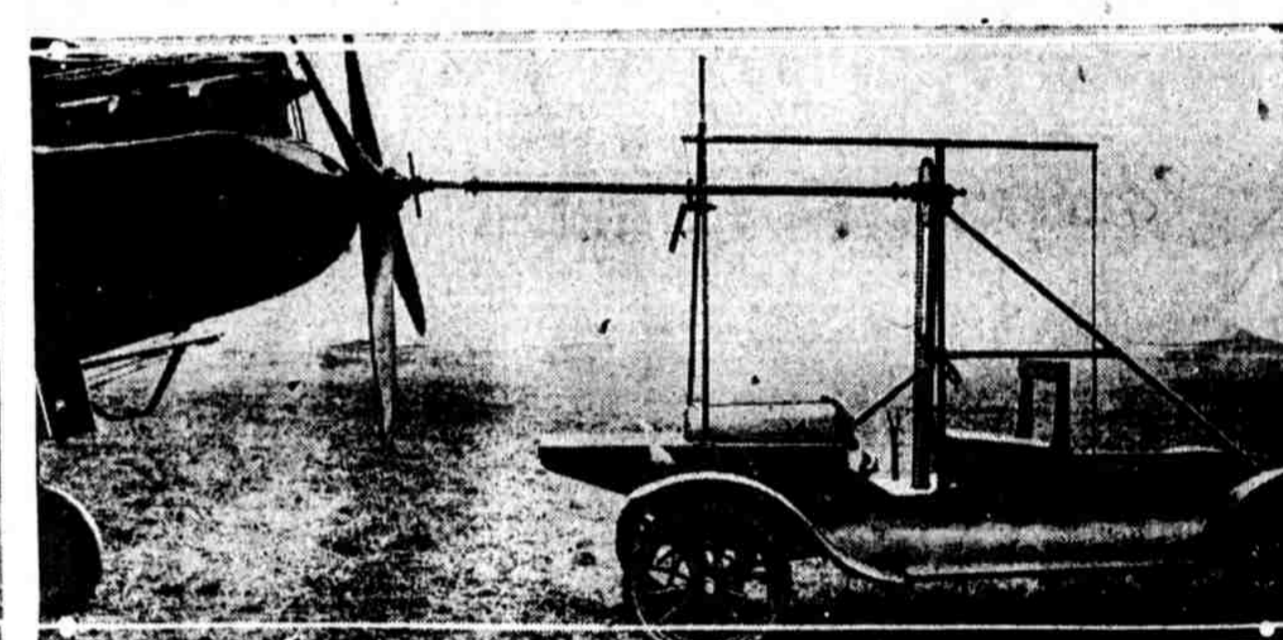
AN AIRPLANE ENGINE STARTER attached to engine of an automobile, originated by Captain B. C. Hucks, a British pre-war pilot.
