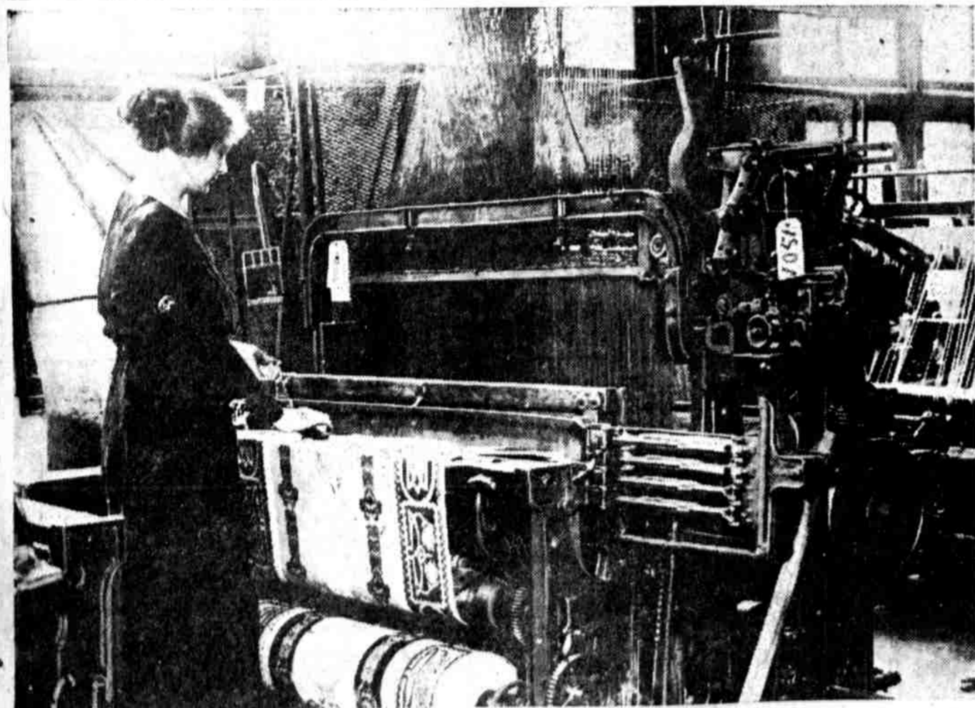
WEAVING HAMMOCK CLOTH at the Hohlfield Manufacturing Co., Tenth street and Allegheny avenue. The loom operator is Miss Selma Koenig, 987 West York street.
