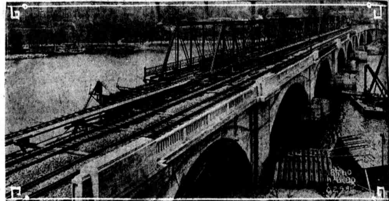
THE NEW concrete Columbia bridge of the Philadelphia and Reading Railway Co. in Fairmount Park. The old iron bridge, in use for thirty-two years, is being taken away, while the finishing touches are being put to the new structure.
