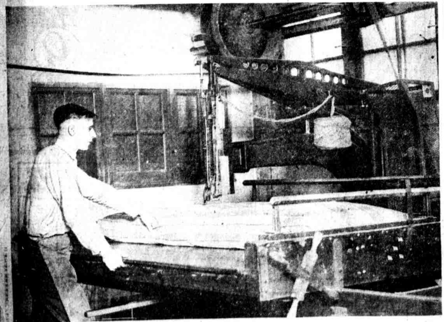
ELWOOD BANKS, 512 West Indiana avenue, operating a tufting machine at the Hohfeld Manufacturing Company, Tenth street and Allegheny avenue. The machine puts tufts on the top and bottom of mattresses and ties them in their place at the same time. This does away with hand work in the making of the mattress.
