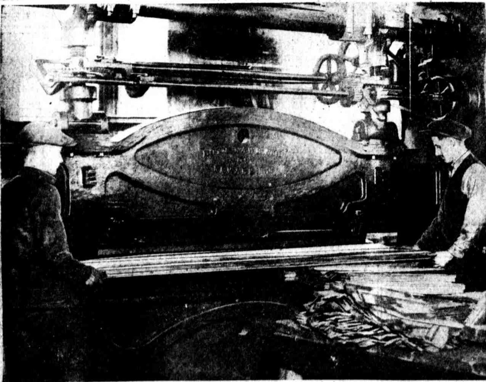
FORMING AND CUTTING bulkhead plates for Hog Island ships at the plant of the International Metal Manufacturing Co., Wayne avenue and Berkley street. Two operators are necessary to handle the machine and the heavy steel. At the left is George Hotter, 2535 North Franklin street, and at the right, Ned Krelhoefer, 2315 West Agate street.
