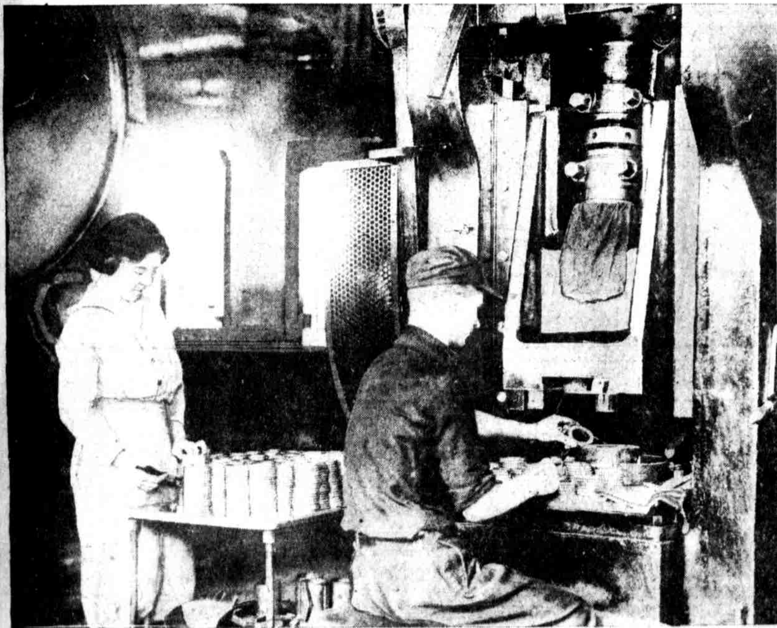
JOHN ZELIK, 2239 Ruffner street, operating a 400-ton pillar-gear press at the Nice Ball Bearing Co., Thirtieth street and Nicetown lane. With this great pressure grooves are pressed into the thrust washers that are used with the steel ball bearings. Miss Elsie Frantz, 2468 West Thompson street, is preparing the washers for the press
