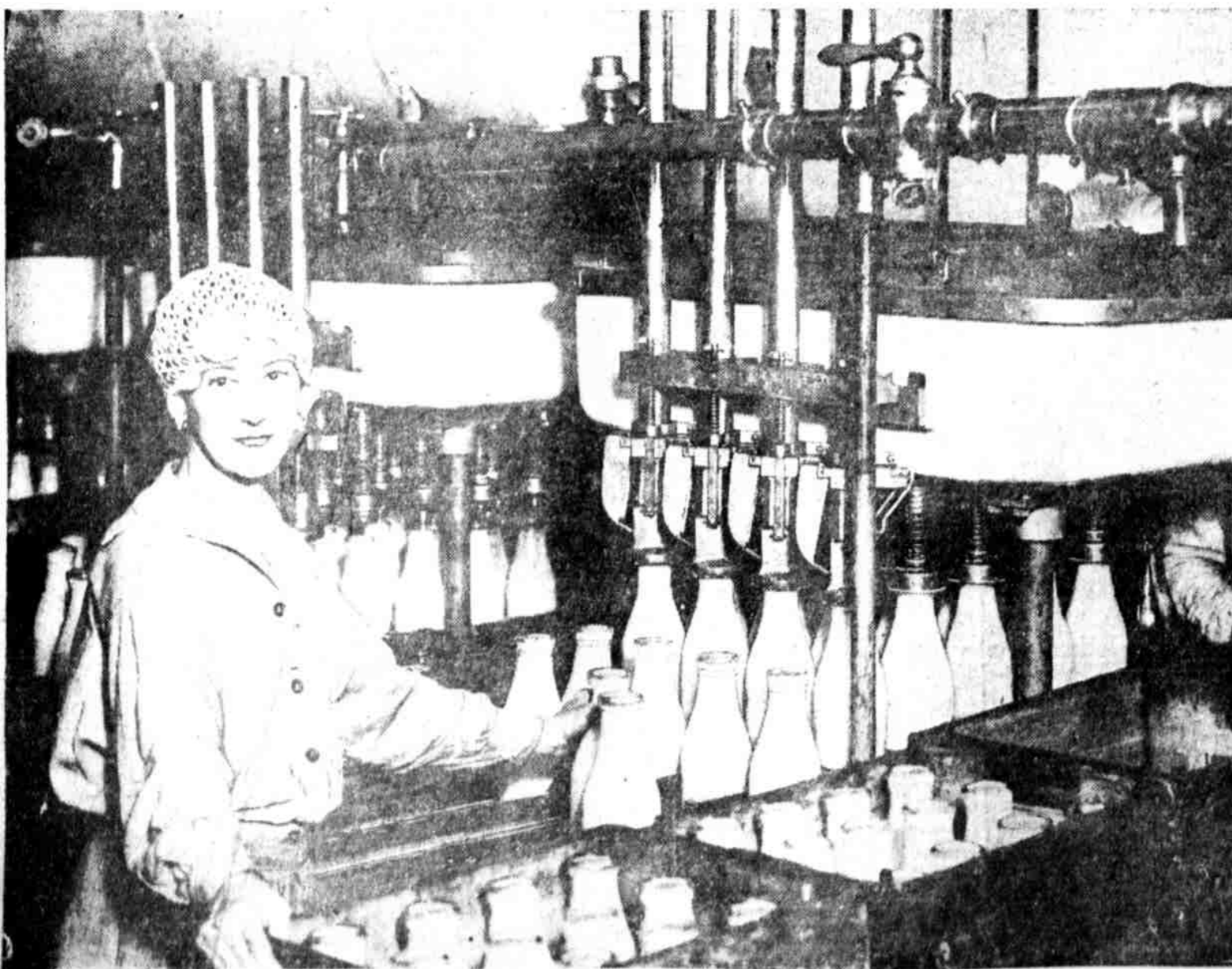
THIS COMBINATION machine fills and caps milk bottles at the milk depot of Supple-Wills-Jones Milk Company, Twenty-sixth and Jefferson streets. The operator is Miss Kitty Miller, 1323 North Twenty-seventh street. She, when bottles are filled and capped, places them in the boxes, which are taken away on a moving belt to the refrigeration room.
