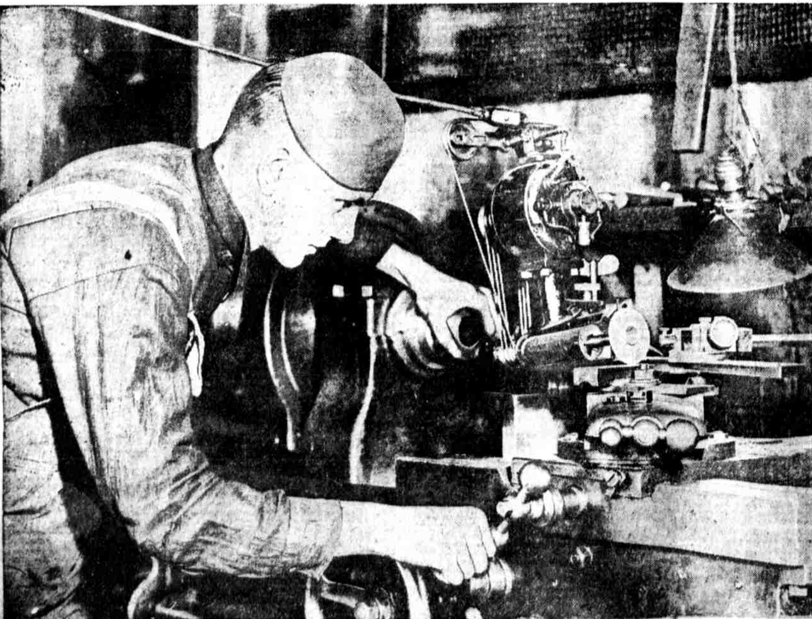
Louis J. Dower, 440 Olive street, is operating a thread-grinding machine at the factory of the Precision and Thread-Grinding Manufacturing Co., 1932 Arch street. By this machine threads are cut into bolts, water taps, dies, etc. One thread to 225 threads per inch can be cut.
