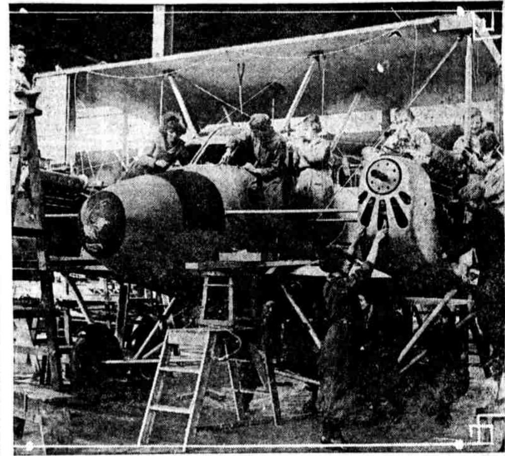
PUTTING THE finishing touches to the "Eagle," the new Curtiss ten-passenger bi-motored airplane. It will be exhibited as the first flying machine to be built mainly by women.
