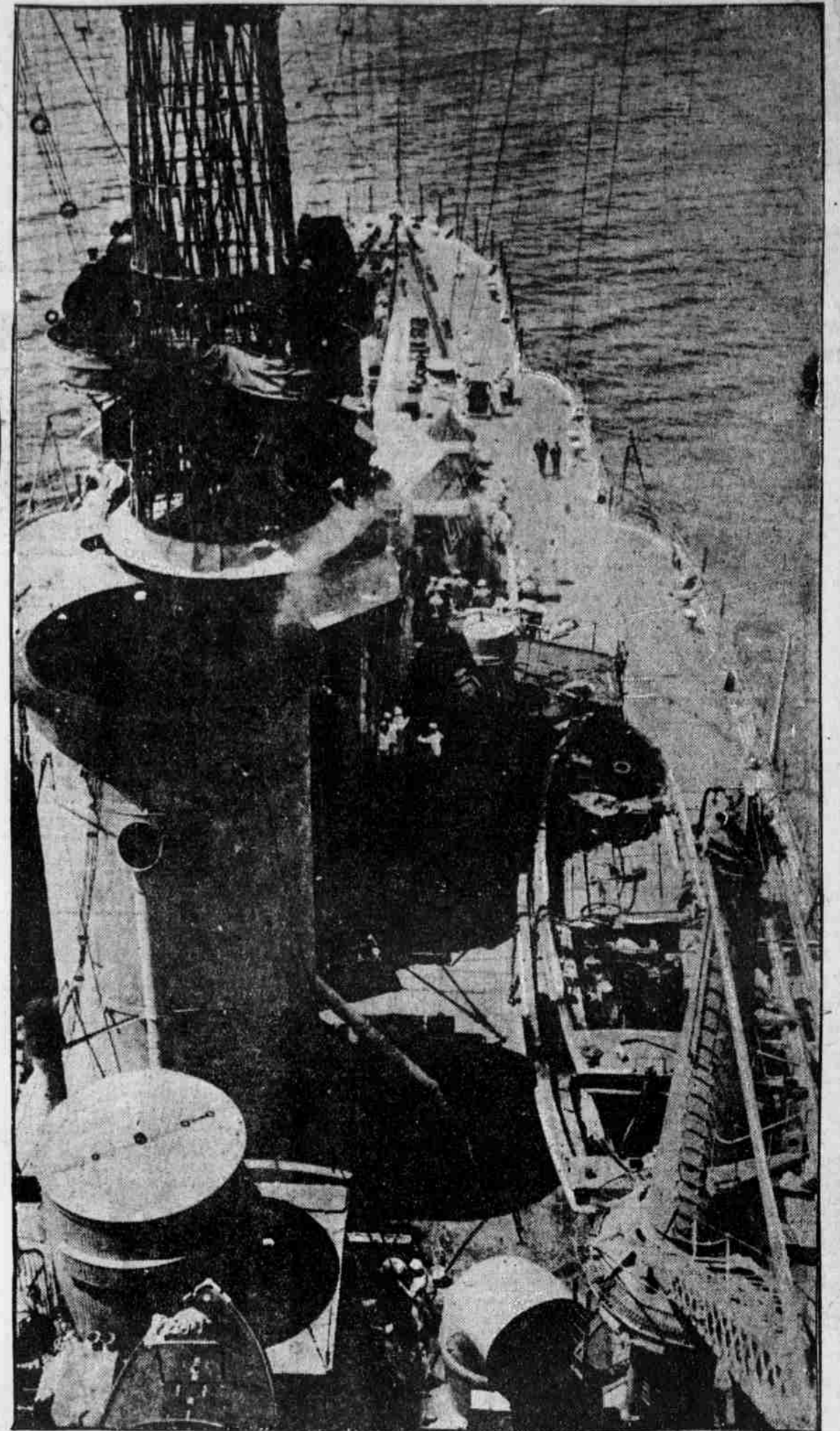
THE U. S. S. NEW MEXICO, flagship of the Pacific fleet—an excellent and comprehensive view of the battleship's deck arrangements and details of construction, photographed from the top mast
