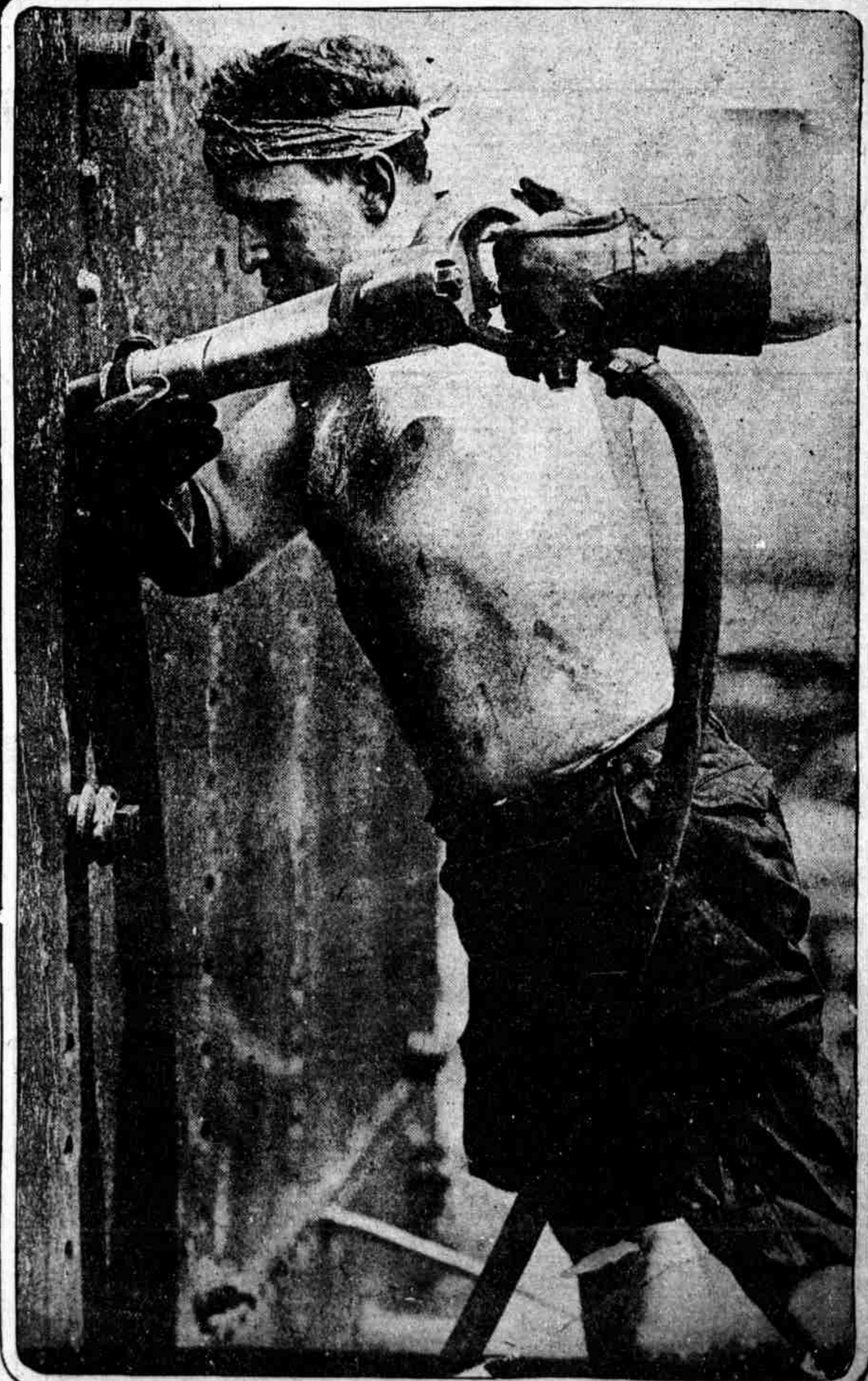
DRIVING WHITE-HOT RIVETS with the temperature at 103 degrees. A man's size job any day and a superman's job on a hot day. But whether the weather is sweltering or freezing, there's no let-up at Hog Island when the call is for speed.
