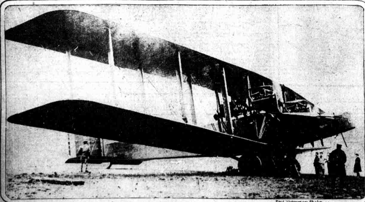
THE GREAT FOUR-ENGINE HANDLEY PAGE MACHINE entered for the transatlantic air race. The view shows the huge dimensions of the airplane which will strive for the £10,000 Atlantic flight prize.
