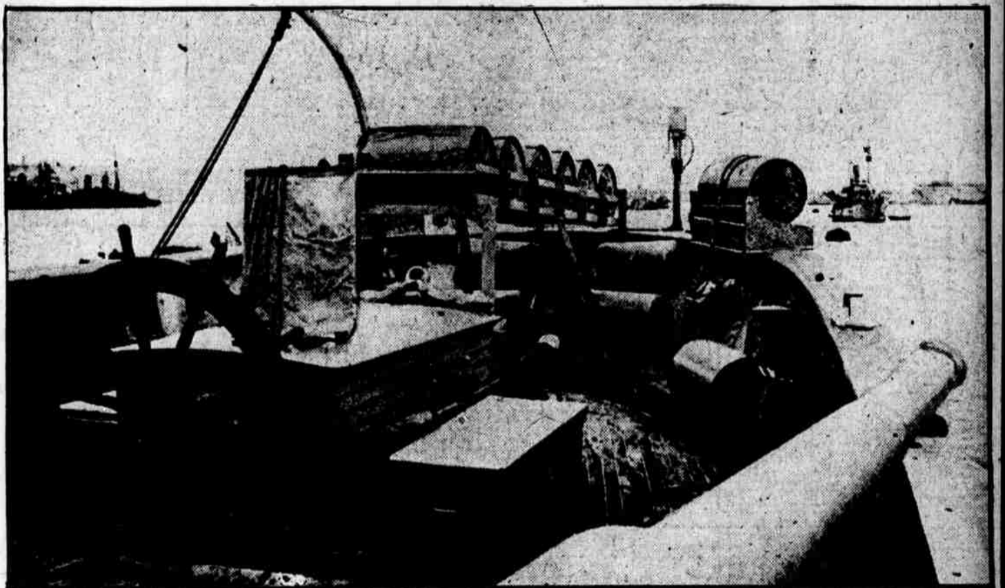
THE U-BOATS' NEMESIS is the depth bomb, with its deadly charge. The photograph above shows how the bombs are ready for release at a second's notice. A sharp incline sends them rolling into the sea. Underwood & Underwood
