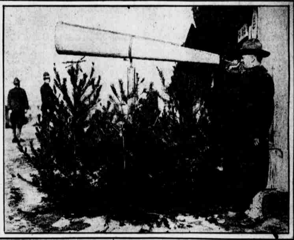
A Regimental Megaphone at Camp Meade, by Means of Which Bugle Calls Are Magnified to Carry Great Distances Across the Cantonment.
