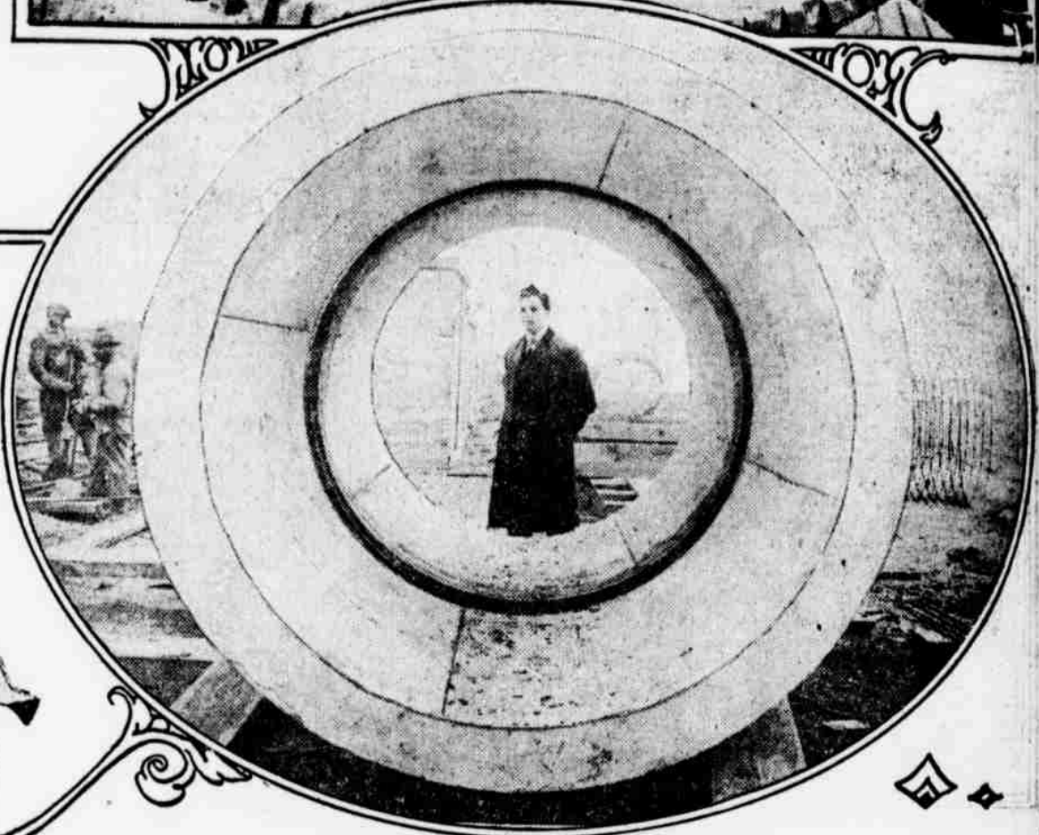
MAMMOTH SEWER FOR "A GREATER PHILADELPHIA" It is the great Frankford Creek Intercepting Sewer, an uncompleted section of which is shown in the upper photograph. Below is one of the 6600 sections of pipe which it will be necessary to use.
