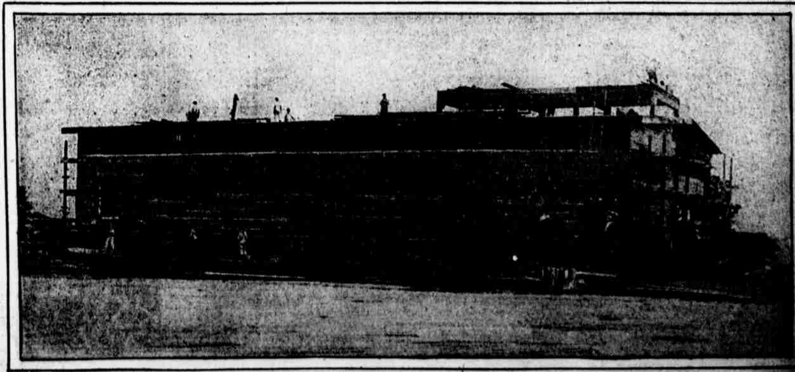
Photograph by General Photo Service. RUSHING WORK ON THE REFRIGERATING PLANT AT WRIGHTSTOWN CANTONMENT In this building, which is nearly completed, will be made the ice needed for food preservation and other purposes of the army base which Uncle Sam is assembling at Camp Dix in the State across the Delaware.
