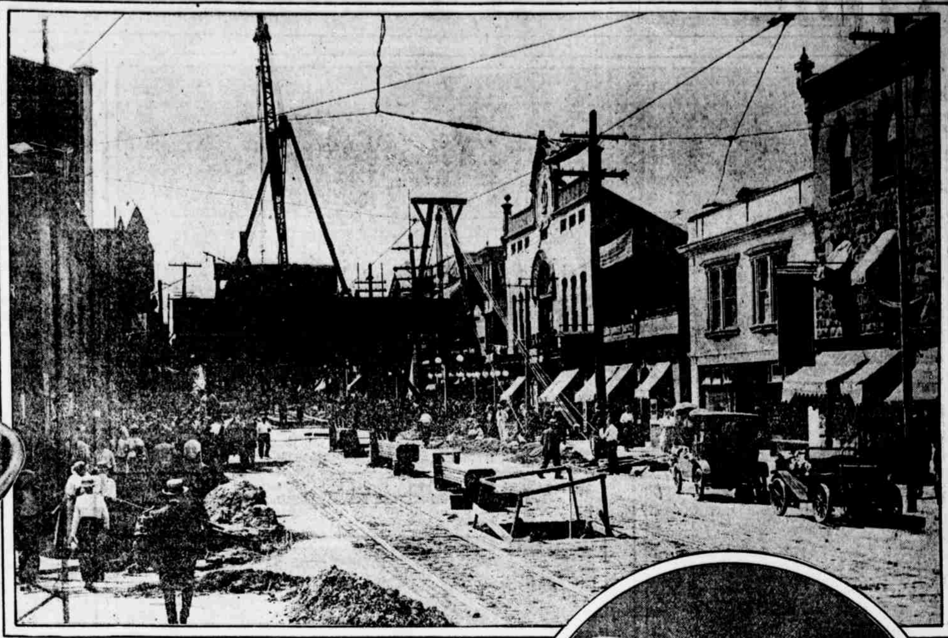
PLACING HEAVY CROSS GIRDERS AT OVERINGTON STREET FOR THE FRANKFORD ELEVATED
