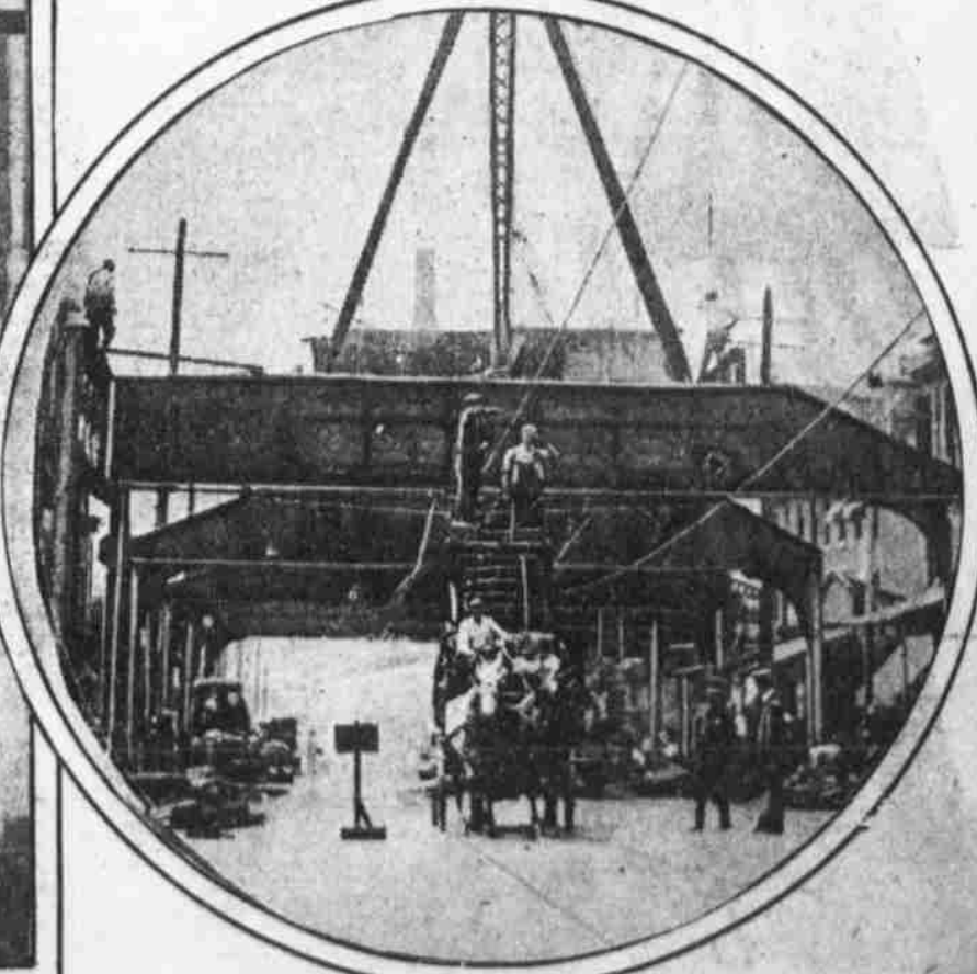
NORTHEAST PHILADELPHIA IS HAVING ITS DREAM OF RAPID TRANSIT The structural work on the Frankford elevated line at present has reached a point near the intersection of Ruan street and Frankford-avenue and the immediate road at Bridge street now looms into sight.
