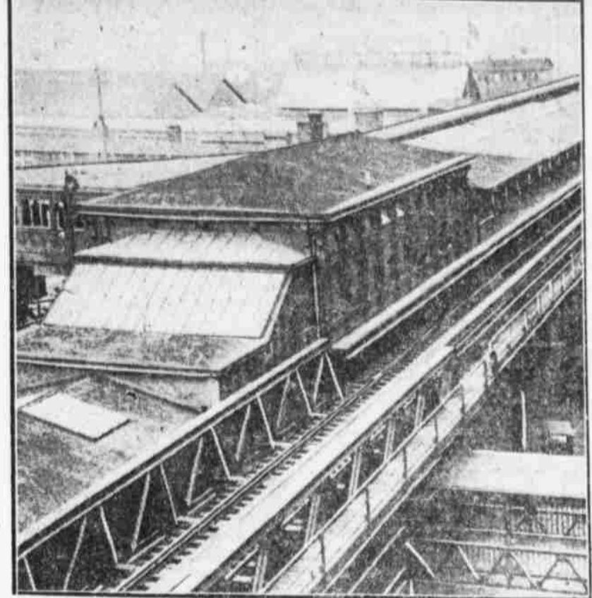
Bids for the construction of five stations along the Frankford elevated line will be advertised by Director Twining next Monday. The type of structure for these stations is illustrated above, while beside it is shown the Market Street Ferry station of the present subway-elevated line, with which the Frankford "L" will connect at Arch street.
