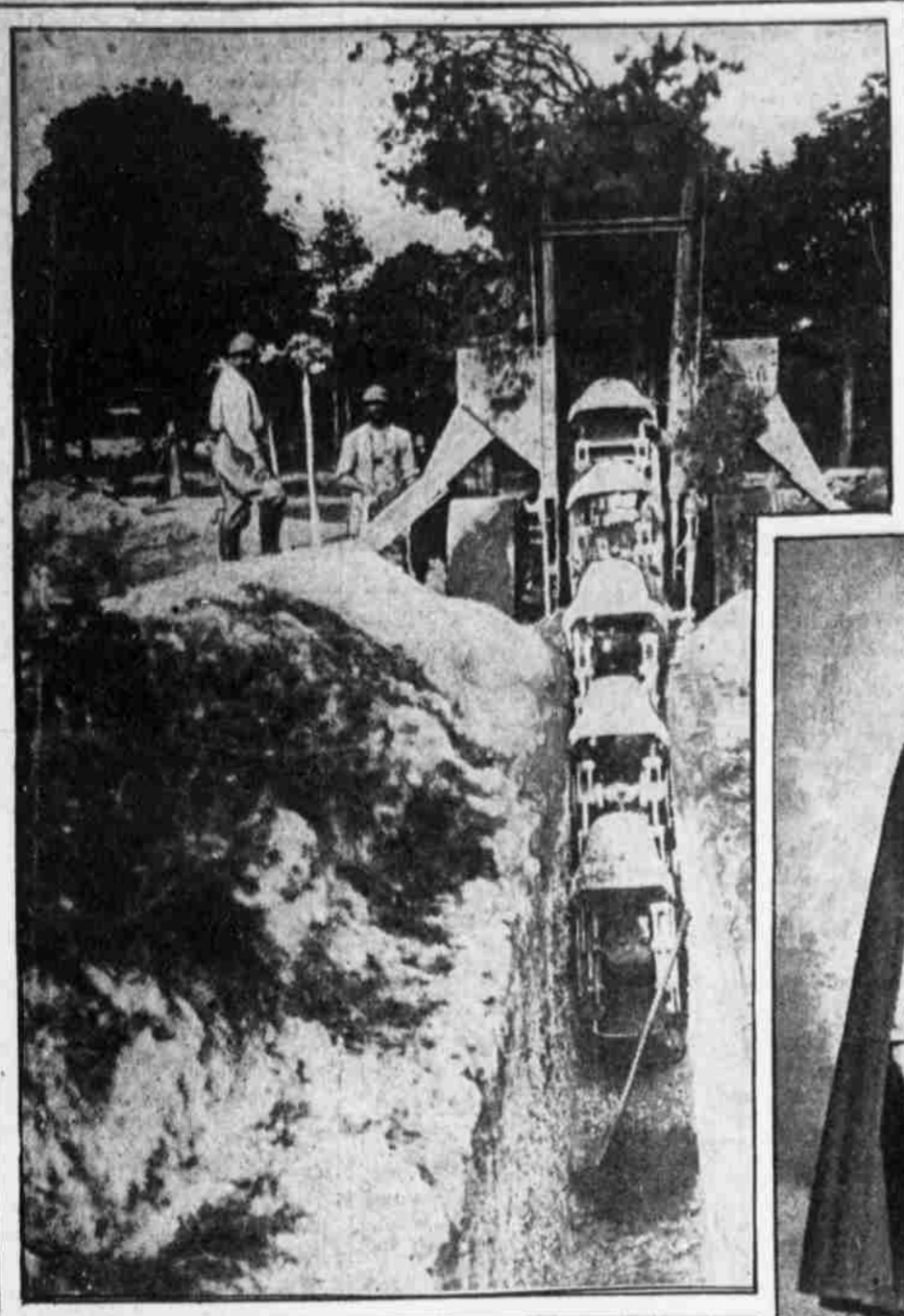
GIANT EXCAVATORS DIG ALLIES' TRENCHES. Much has been said about the machines used by the Germans for trench digging, but they have been surpassed by the British and French implements, which cut the trenches and build the parapets at the same time.
