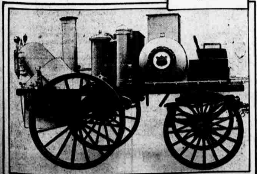
UNCLE SAM'S BOYS ENJOY PURE WATER IN THE FIELD Sterilizable sterilizer, designed by a Philadelphia firm, is the answer to the problem of getting drinking water.
