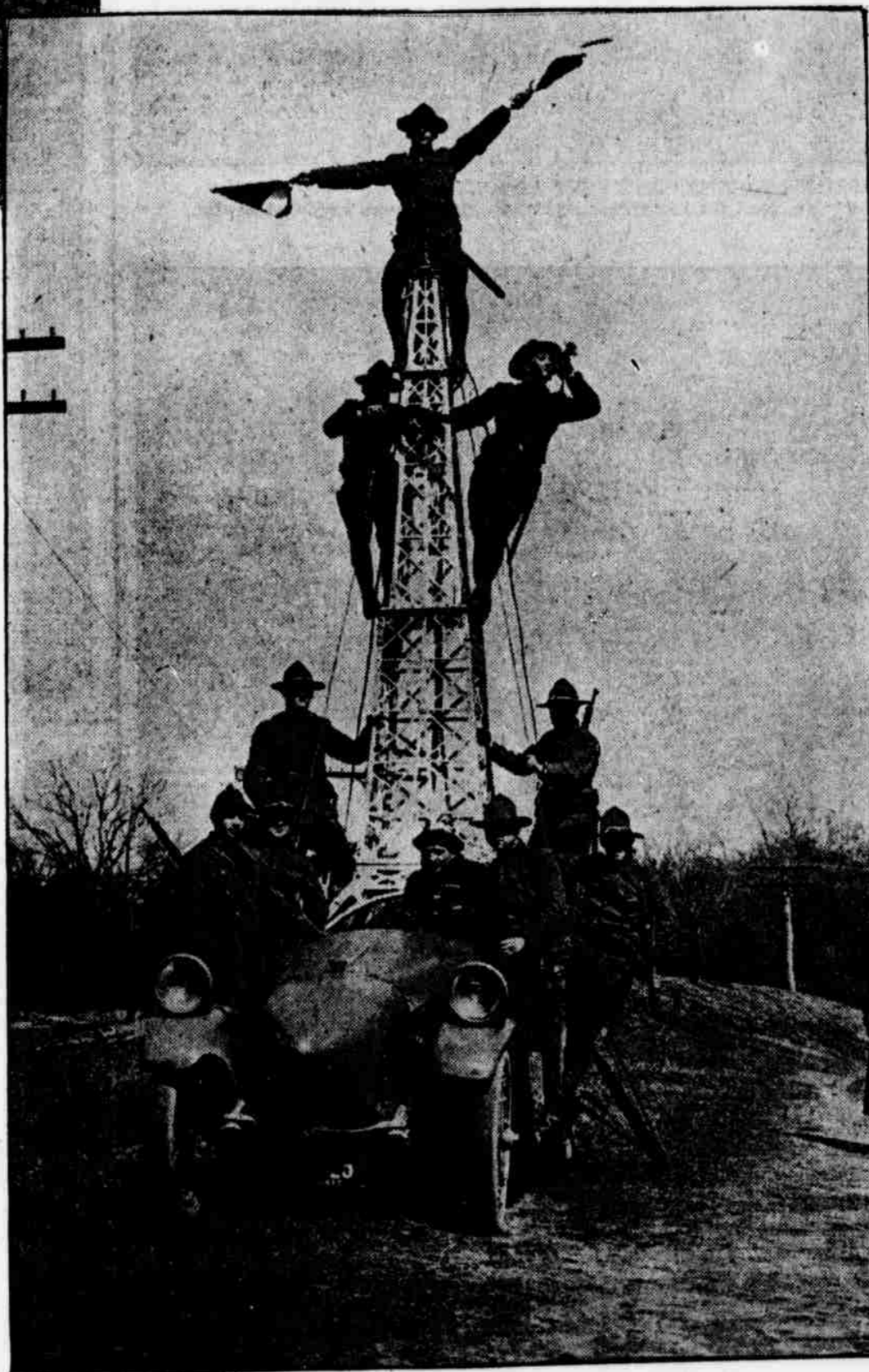
Copyright, American Press Association. NEW MILITARY DEVICE HAS MANY USES Steel tower mounted on armored automobile, which can be employed for signalling, observation, outpost station work and in military field wireless. The United States army is being equipped with them.
