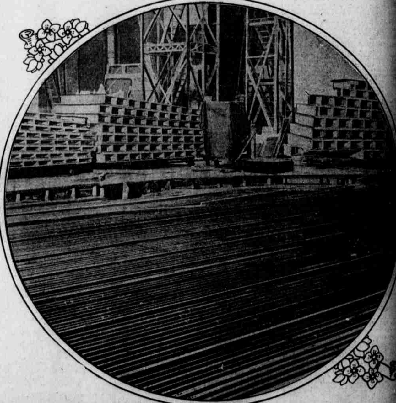
HOW AN ICE POOL IS MADE FOR THE BIG THEATRICAL SKATING SCENES A section of the stage flooring is lifted out and the bottom of the hole is lined with pipes filled with certain chemicals. Then water is turned on, and there you are. This is what the Hippodrome show has done to the dignified stage of the Metropolitan Opera House.
