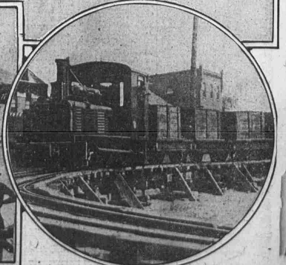
BALDWIN'S TURNS OUT TRENCH TRAINS FOR RUSSIA This is a picture of the 50-horsepower gasoline engine designed to haul ammunition and supplies to the fighting line and a type of the cars to be used.
