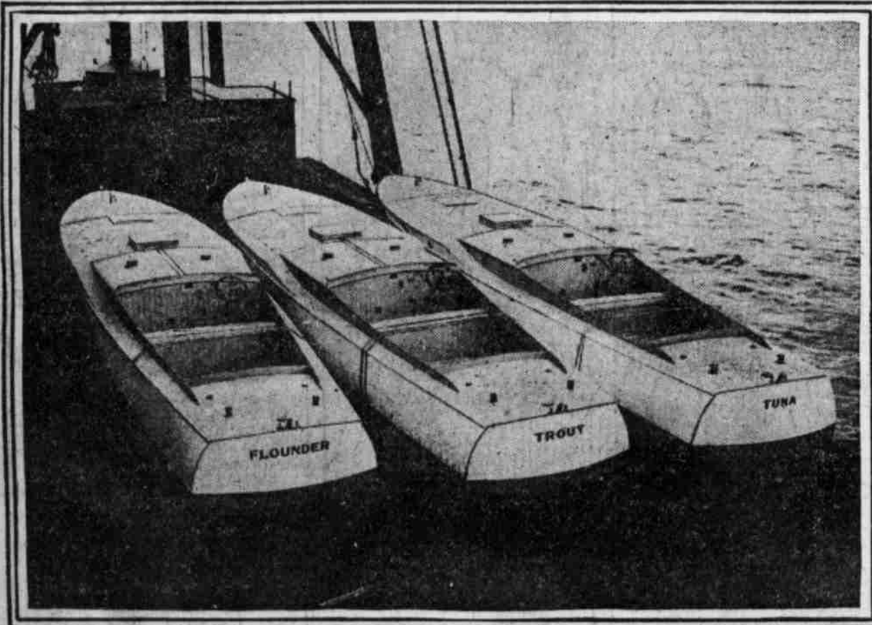
AMERICAN-BUILT SUBMARINE CHASERS FOR THE BRITISH NAVY Photo by Medem Service These gasoline, 100-horsepower launches were constructed at South Boston, Mass., at a price of $4000 each. They will carry a three-inch gun forward and make about 25 knots an hour. They require only two men to man them.
