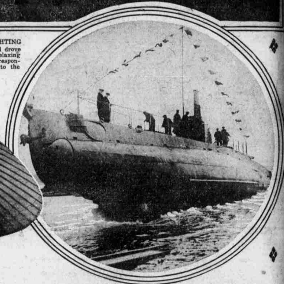
LAUNCHING OF THE NEW BRITISH SUBMARINE H-5 AT THE FORE RIVER SHIPBUILDING COMPANY, QUINCY, MASS. One of the 10 submarines being built for the British navy by the Fore River branch of the Bethlehem Steel Company, to be delivered after the war.
