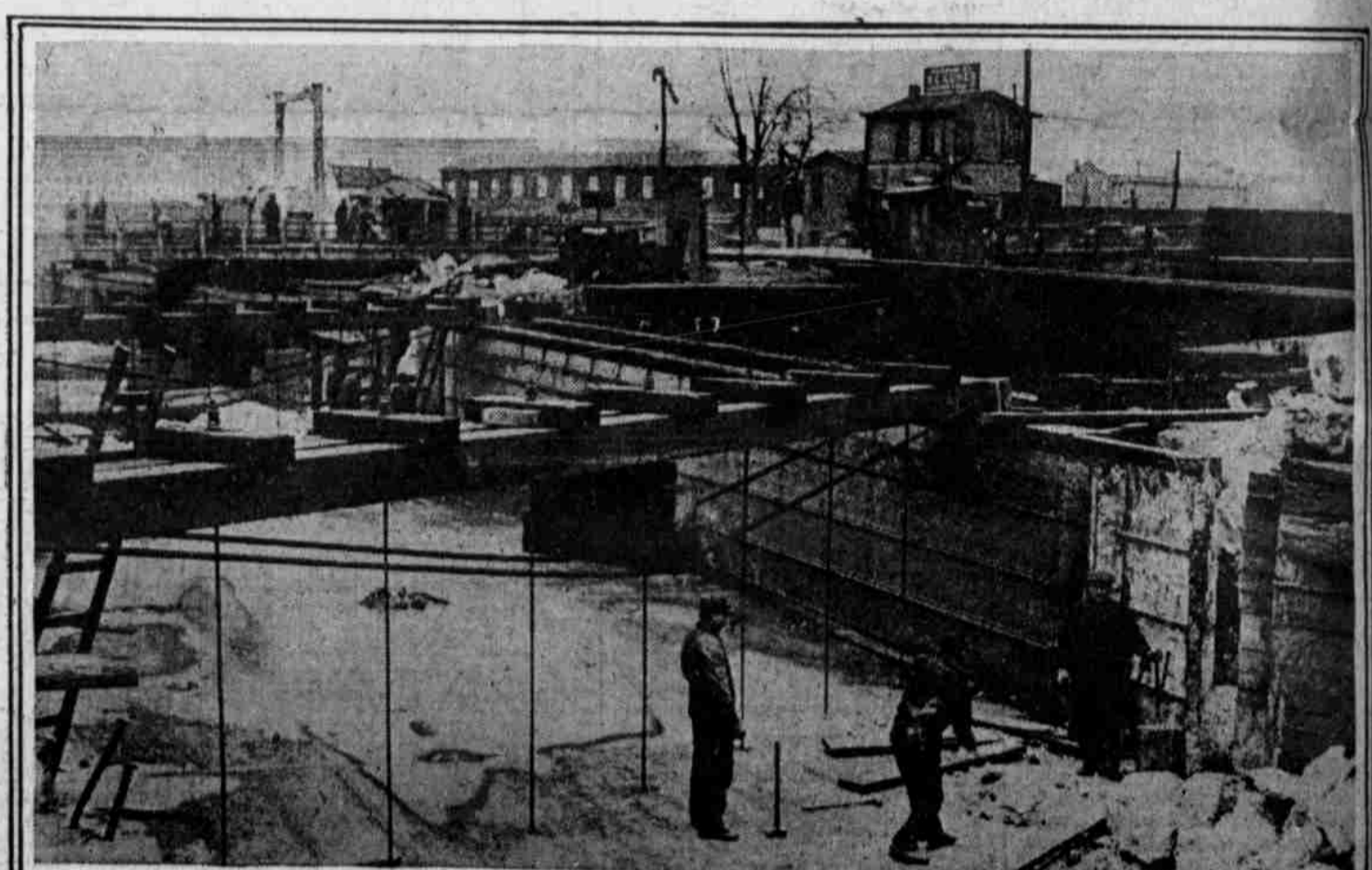
WHERE A CANAL INTERFERED WITH A RAILROAD BELOW At Trenton, N. J., the level of the Delaware and Raritan Canal is being raised to permit the largest locomotives of the Pennsylvania Railroad to pass through the tunnel beneath. Usually railroads prefer to pass over a canal instead of under it.
