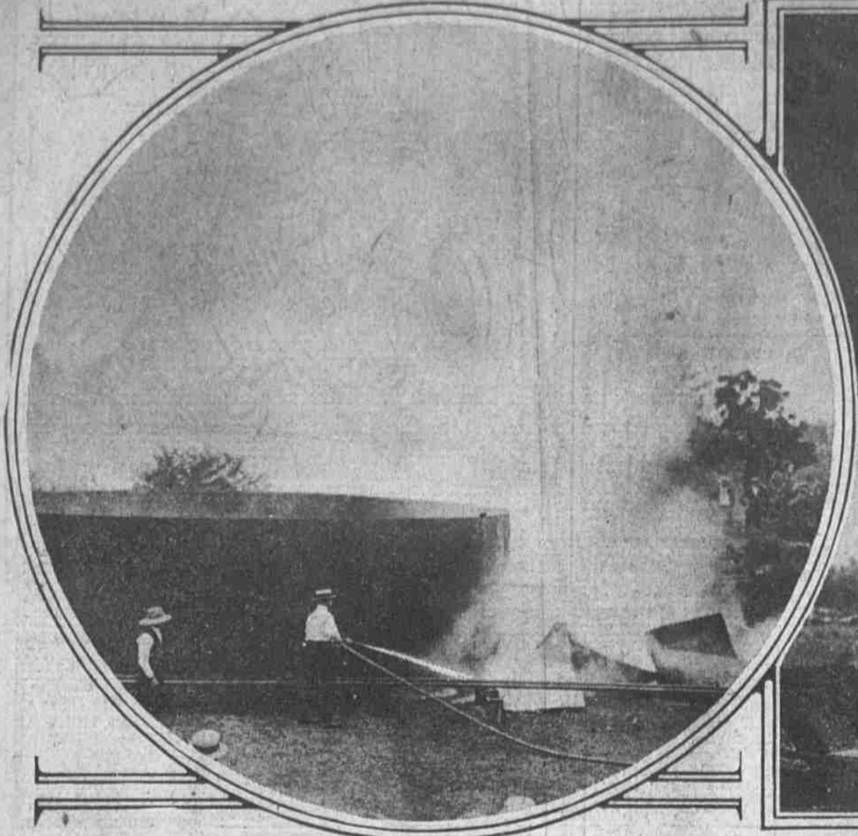
PUTTING OUT A BLAZE IN AN 80,000-GALLON OIL TANK WITH A SLENDER STREAM FROM A HOSE FULL OF LICORICE JUICE A test was made at the plant of the Crew-Levick Company, in Chester, Pa., yesterday of a new chemical invention by W. W. Walker, of Camden. A lighted paper was thrown into the tank of inflammable liquid, which instantly burst into flames with characteristic heavy, black volumes of smoke, as shown on the right. Into the mess the inventor then turned his hose of "licorice juice," as he called it, and within a few minutes both flame and smoke were entirely conquered, as shown on the left. The inventor contends that his discovery will cause a revolution in old methods of fighting such fires.
