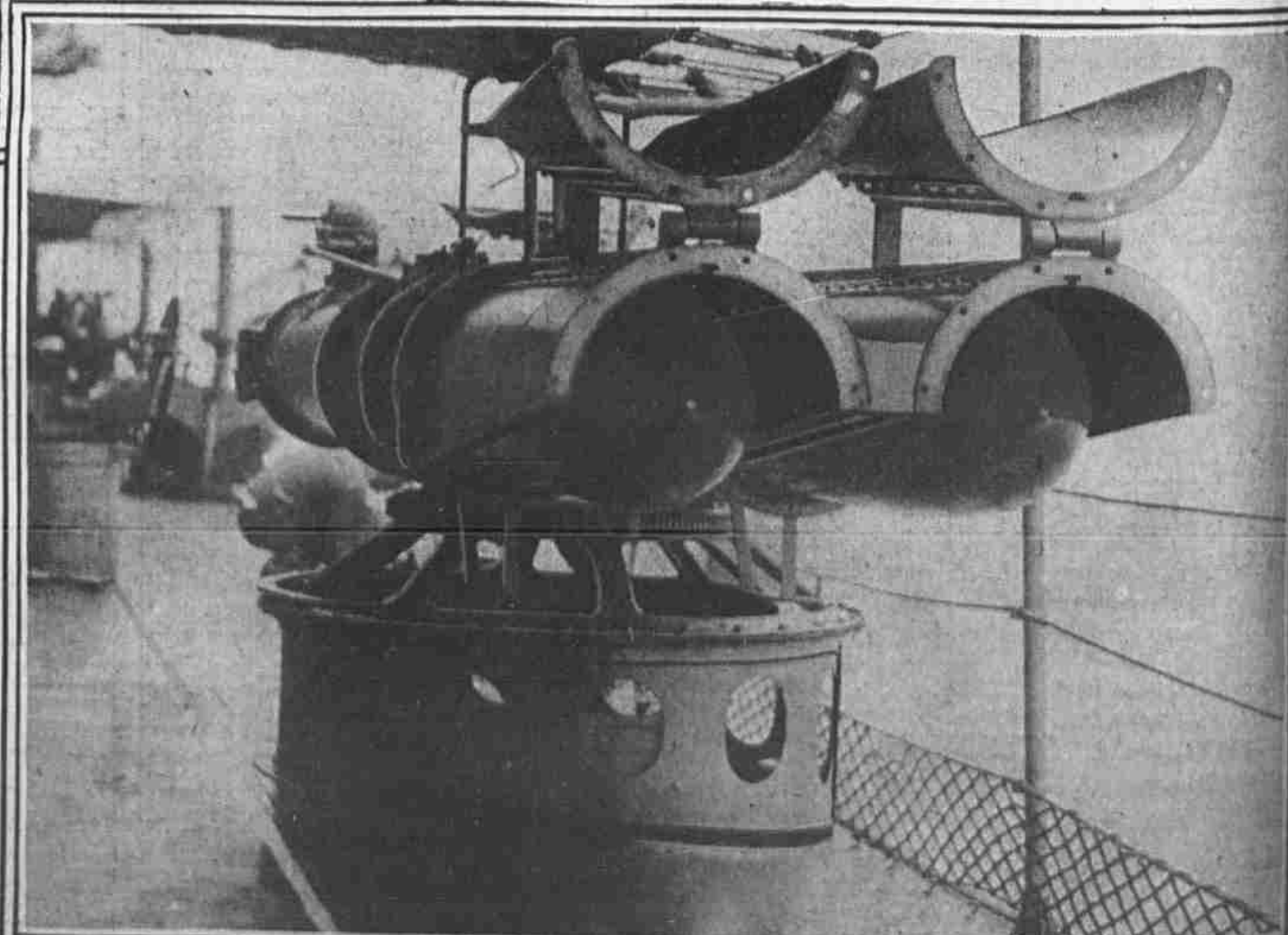
TORPEDOES AND TORPEDO TUBES AS MOUNTED READY FOR ACTION ON DECKS OF BATTLESHIP TEXAS
