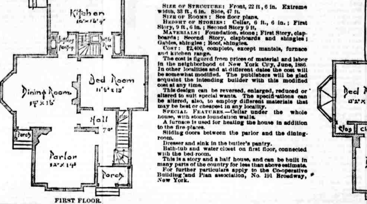
FIRST FLOOR. SECOND FLOOR.
