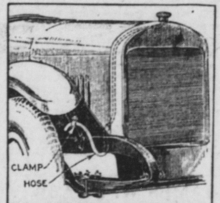
Length of Rubber Tubing, Attached to Overflow Pipe, Disposes of Alcohol Odors.
