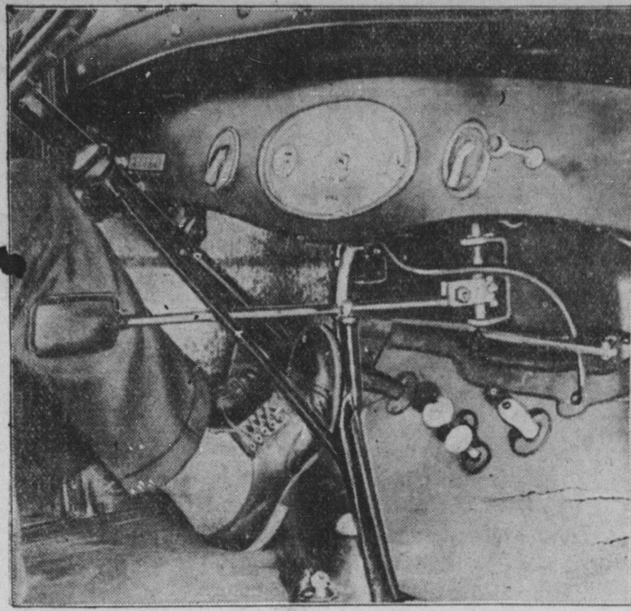
The photograph shows the new invention for safer driving, the leg accelerator. When the driver goes uphill or through dense traffic he can keep his foot on the brake and at the same time manipulate the accelerator with his leg. When not in use, the leg accelerator telescopes under the dash.
