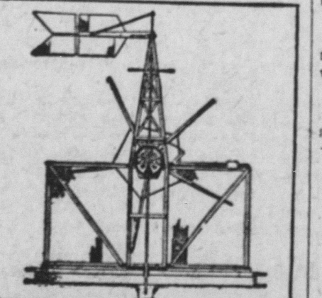
Windmill Provided With Means for Self-Adjustment to the Wind.
