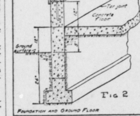
Fig. 2—Showing a Good Method of Making Foundation and Floor of a New Building Ratproof.
