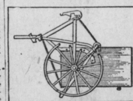
A Side Elevation of the Truck in Position for Beginning to Load.
