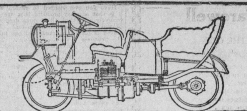
By Placing the Air-Cooled Engine Under the Front Seat, This Automobile, of Japanese Design, Secures a Large Seating Space in a Light Car.
