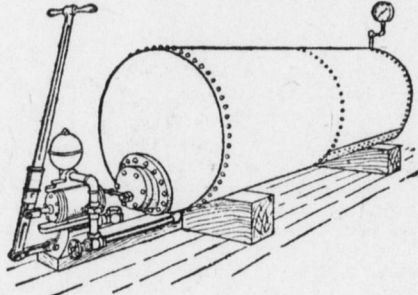
Hand Pump and Pressure Tank.
