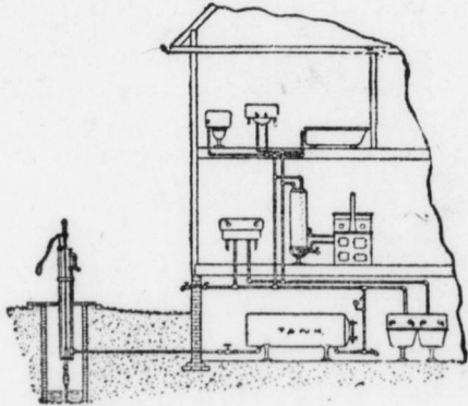
Domestic Water Works System.
