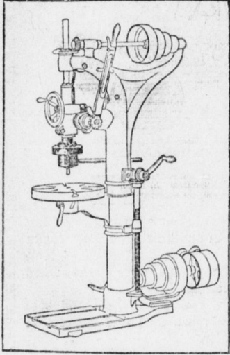
Machine That Makes Square Holes.
