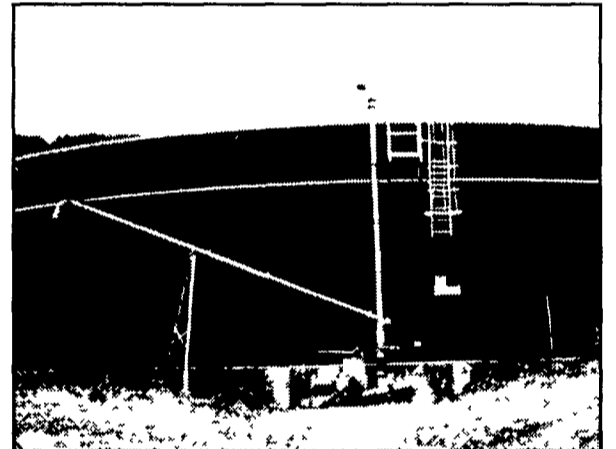
Side-mount Pump with 4,300 gal./min. agitation
