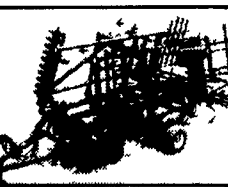
A 25344 SF 6332-20" Land Finisher, 18 5" Blades, 7 5" Spacing, New Sweeps, Center Duals, Cyl/Hoses
