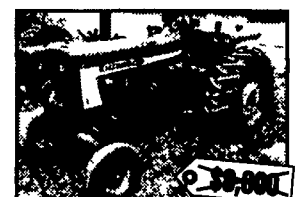
C 43495 IH 756 , 9105 Hours, 540/100 PTO, 3PT Hitch, Rear Weights, 2 Remotes, 18 4x34 Rear Tires, New Clutch, 76 HP
