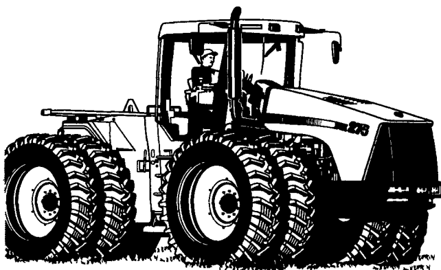
B 43937 1997 CIH 9390 4WD Cab, 3739 Hours, Front & Rear Duals 20 8x42, Manual Transmission, 4 Remotes, 425 ENG HP
