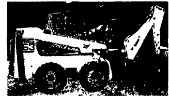
2001 BOBCAT 763 G-Series w/709 backhoe attach w/quick attach bucket, rear stabilizers front & rear aux Hydros suspension seat, new 68" lo-pro bucket, counter weights, foam filled tires @ 75%, Kubota Diesel only 625 hrs Outstanding Condition ONLY $19,995
