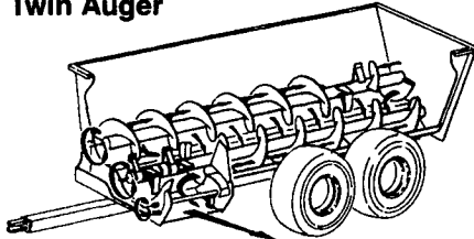
Cut-away view showing Patented Material Flow
