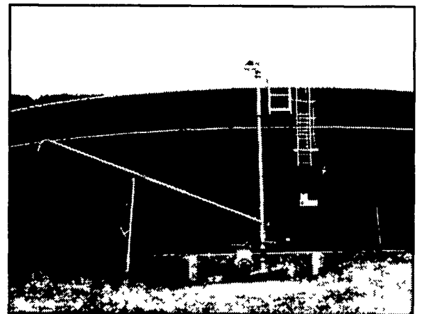
Side-mount Pump with 4,300 gal./min. agitation
