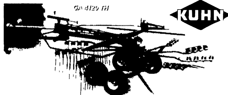
GA4120 TH 10 Pt. 6 Inch Clean Rake
