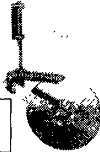
Generation III Fertilizer Coulter Fert Coulter Rear Knife $336.00 Fert Coulter H D Spring Inj $356.00 No-Till Coulter (Shown) $280.00* * Plus Choice Of Blade, Shank & Mtg Kit
