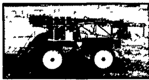
B 42442 Wilmar 7400 Sprayer, Only 1 1/2 Years Old, 225 Hours, 90' Boom, Mid-Tech Monitor, 750 Gallon Tank, Foam Marker, Articulated
