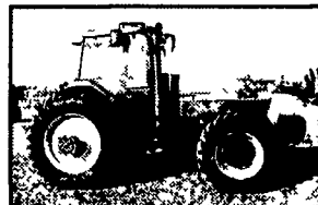
B 43058 1998 CIH 8940 MFD Cab, 1904 Hours, Tires Fr-16 9x30, Rear-20 8x42, 3 Remotes, 1000 PTO, 3 Pt Hitch, 205 HP
