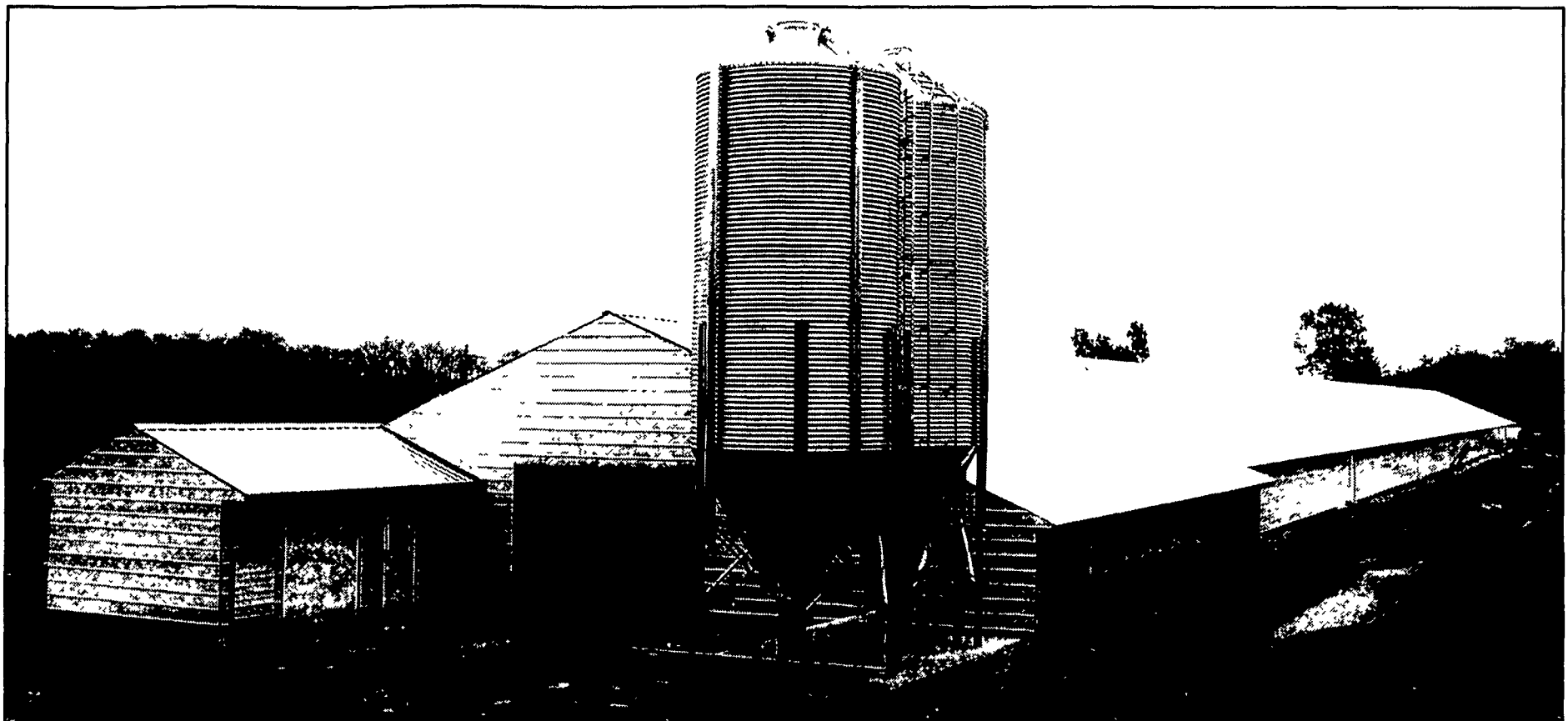
44x500 Tunnel Ventilated Broiler House
