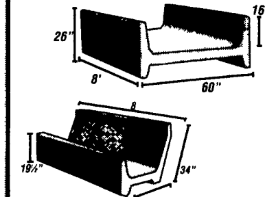
Concrete Feed Bunks
