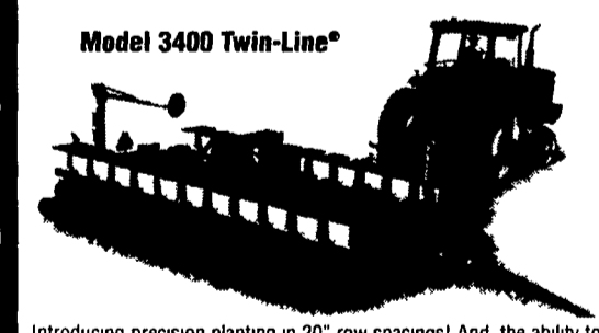
Model 3400 Twin-Line® Introducing precision planting in 20" row spacings! And, the ability to plant ultra-narrow 10" or 11" rows with the KINZE® Interplant® System Plus, in-line transport as narrow as 11"3" (12' 7" with the Interplant® Package and no till coulters)
